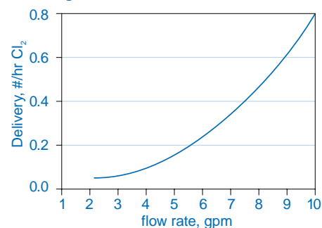
NSF Delivery Rate for Titan GT100 using Accu-Tab Blue SI tablets
